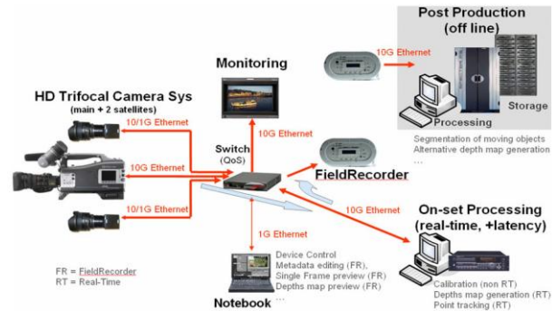
Figure1: 3D capture workflow for the trifocal approach
