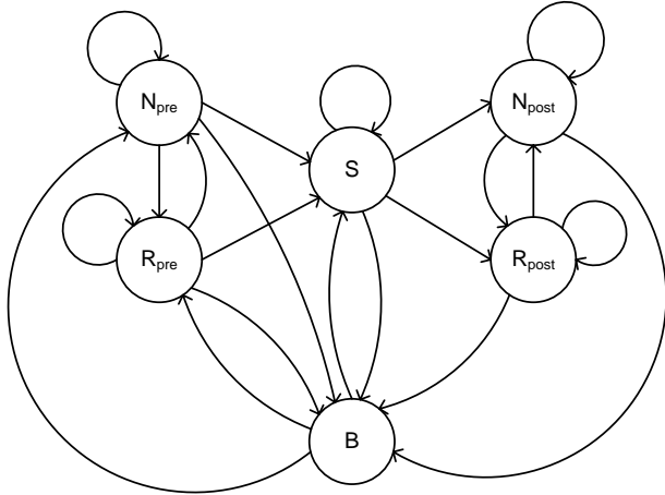
Fig. 1. Topology of the 6 state HMM.
